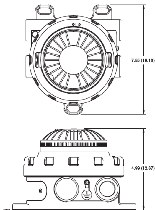
Figure 2—U5015 Dimensions in Inches (cm)
