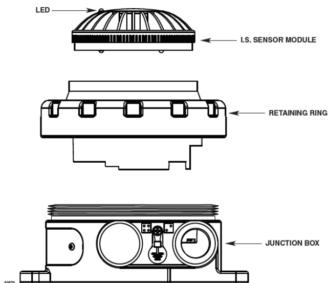
Figure 1—U5015 Components
